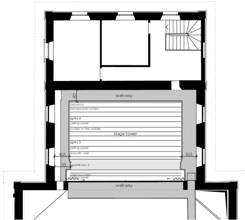
PLAN STAGE TOWER
